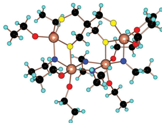
Fig. 3 Molecular structure of [\text{Ti}_4(\mu_2\text{-OEt})_4(\text{OEt})_8(\mu_4\text{-(OCH}_2)_4\text{C})] showing the two fivefold- and sixfold-coordinated titanium atoms. Atom Ti1 (right) adopts an approximate square-pyramidal conformation while atom Ti2 (left) adopts an approximate trigonal bipyramidal coordination. Selected bond distances (pm) and angles ( ^\circ ): \text{Ti-OEt} = 177.0(3)\text{--}181.1(3) , \text{Ti-(}\mu_2\text{-OEt)} = 196.8(3)\text{--}210.6(3) , \text{Ti-(}\mu_4\text{-(OCH}_2)_4\text{C)} = 181.3(3)\text{--}208.8(3) , \text{Ti-OEt-Ti} = 106.0(2)\text{--}109.5(2) , \text{Ti-(}\mu_4\text{-(OCH}_2)_4\text{C)-Ti} = 107.1(2) .
