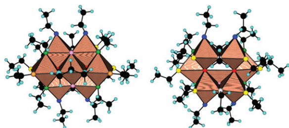
Fig. 2 Molecular structure of [\text{Ti}_7\text{O}_4\{\text{O}(\text{CH}_2)_3\text{O}\}(\text{OEt})_{18}] showing the selective substitution of gem -di- \mu_2\text{-OEt} groups in [\text{Ti}_7\text{O}_4(\text{OEt})_{20}] . (Left) View of the complex with the substituting ligand at the front. (Right) View of the same complex rotated by 180^\circ along the bottom-up direction (substituting ligand at the back).
